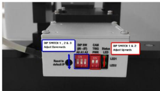
Front Projector Dip Switch Set Up
