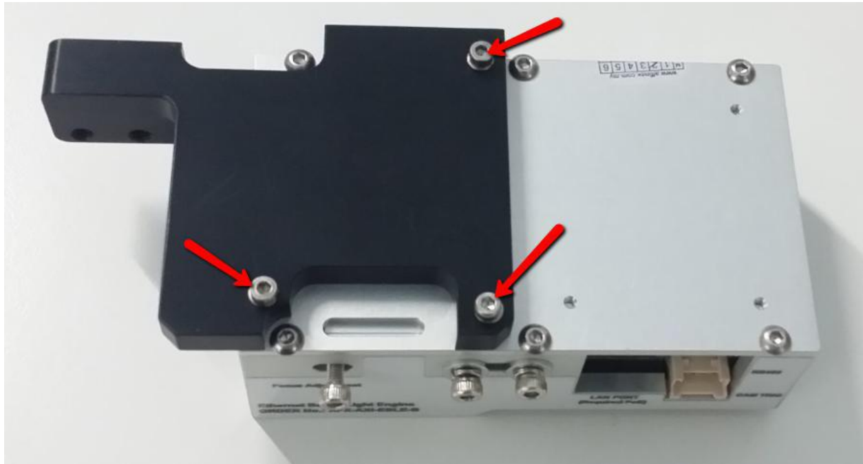
Figure 9 Projector Dismantle
