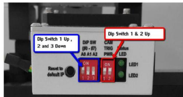
Rear Projector Dip Switch Set Up
